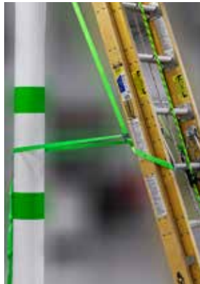
Lower Attachment
